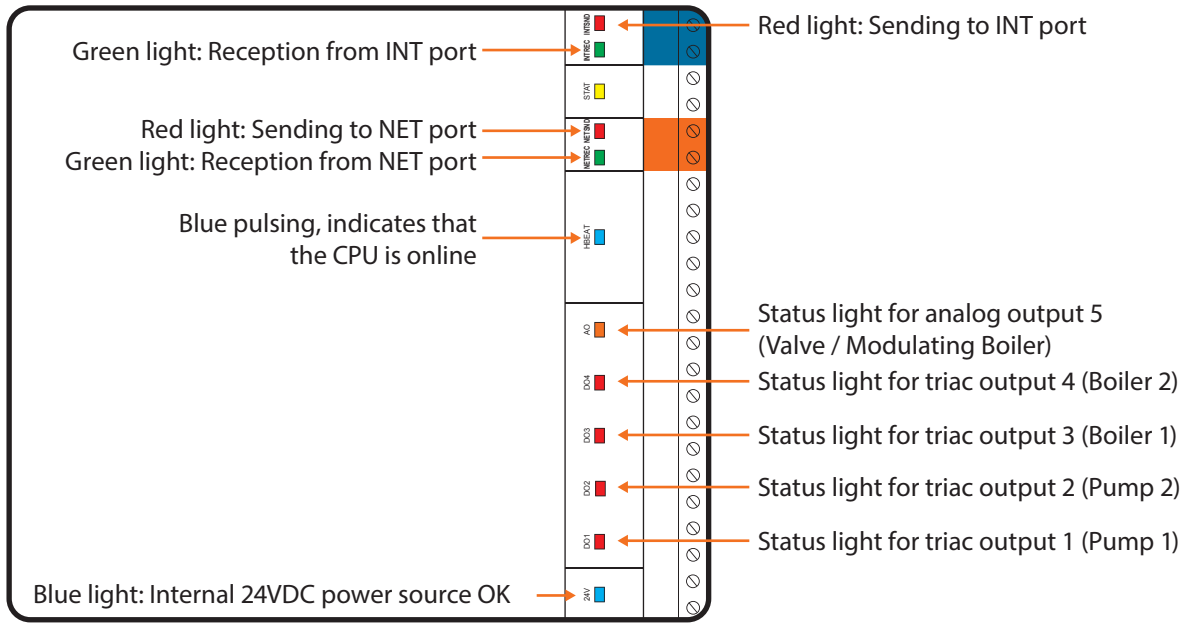
Figure 2 - LEDs Identification
